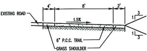
3 TYPICAL SECTION (RURAL) NO SCALE
