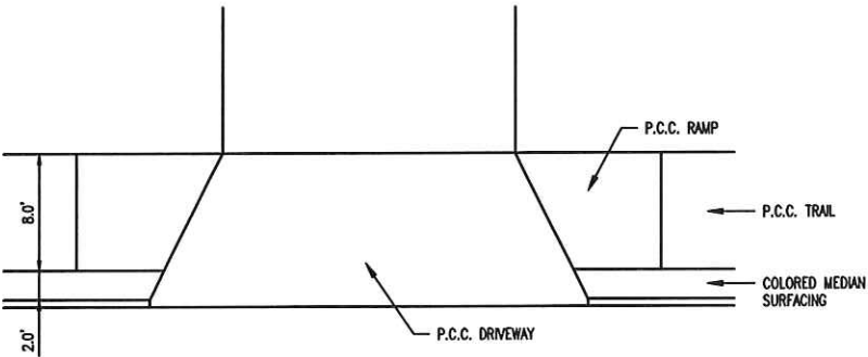
5 TYPICAL DRIVEWAY PLAN NO SCALE
