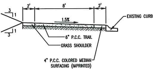
1 TYPICAL SECTION (URBAN) NO SCALE
