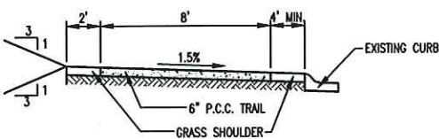
2 TYPICAL SECTION (URBAN) NO SCALE
